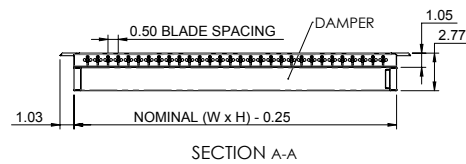
Vertical with Damper
