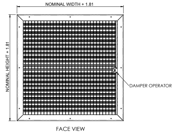
Horizontal with Damper
